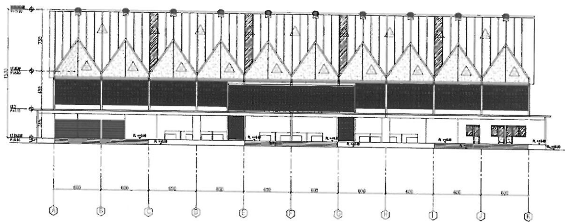
TAMPAK DEPAN/SELATAN/UTARA (VIEW A) SKALA 1: 200
