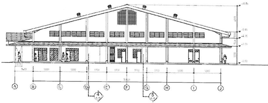
TAMPAK KANAN (VIEW B) SKALA 1:200
